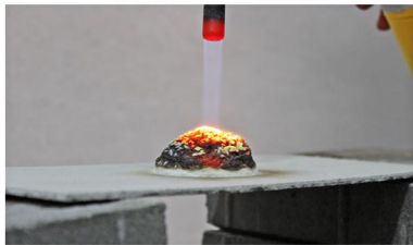
Picture 3 FireShield exhibits up to 50 times volume expansion with continuous fire exposure.
