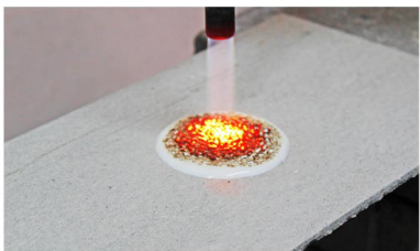
Picture 2 After fire exposure FireShield starts to swell.
